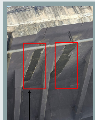
UHPC Joints
